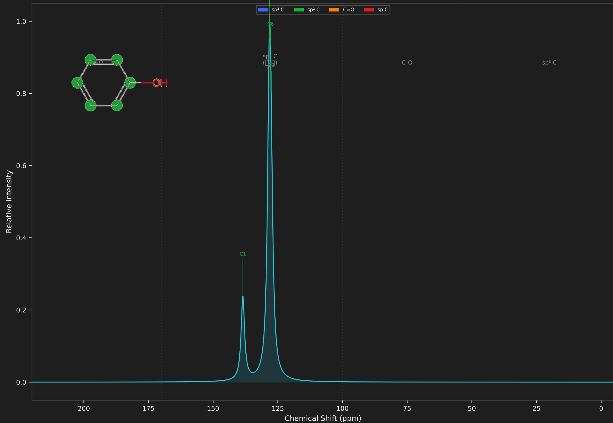
Predicted ^{13}\text{C} NMR Spectrum (SMILES Oc1ccccc1 )
